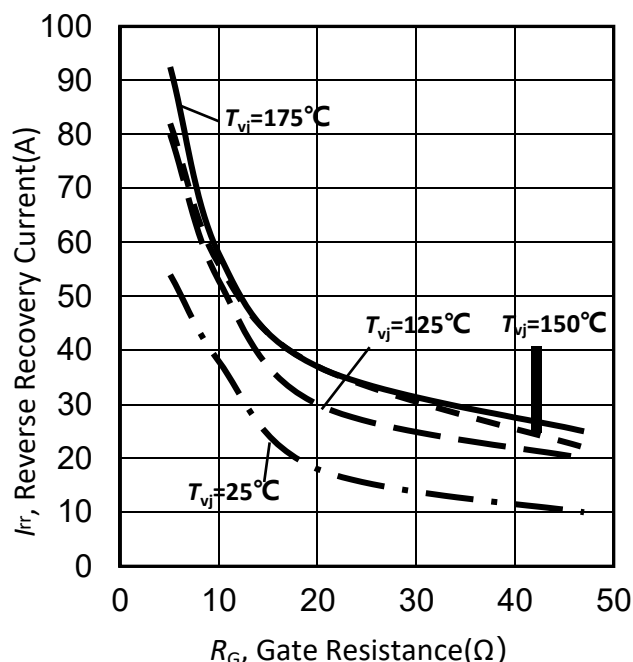
Figure 66. 典型反向恢复电流与栅极电阻器的关系 /Typical reverse recovery current as a function of gate resistor (inductive load, V_{CE}=600V , V_{GE}=-5/17V , I_C=75A )
