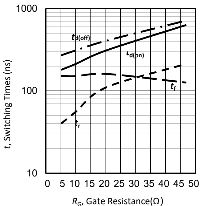
Figure 41. 典型开关时间与栅极电阻器的关系/Typical switching times as a function of gate resistor (inductive load, T_{vj}=150^{\circ}\text{C} , V_{CE}=600\text{V} , V_{GE}=-15/15\text{V} , I_C=75\text{A} )
