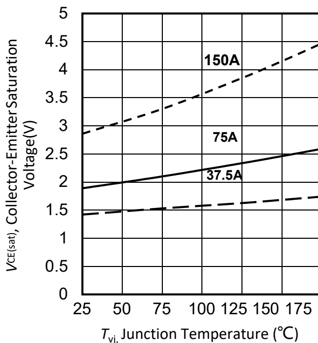
Figure 6. 典型 V_{CE(sat)} - T_j 特性曲线/ Typical V_{CE(sat)} - T_j characteristic ( V_{GE}=15V )
