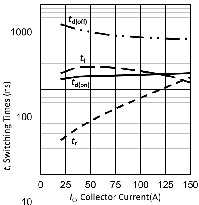
Figure 31. 典型开关时间与集电极电流的关系 /Typical switching times as a function of collector current (inductive load, T_{vj}=175^{\circ}\text{C} , V_{CE}=600\text{V} , V_{GE}=-5/17\text{V} , R_G=10\Omega )
