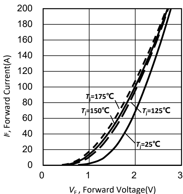
Figure 53. 典型二极管正向电流与正向电压的函数关系/Typical diode forward current as a function of forward voltage
