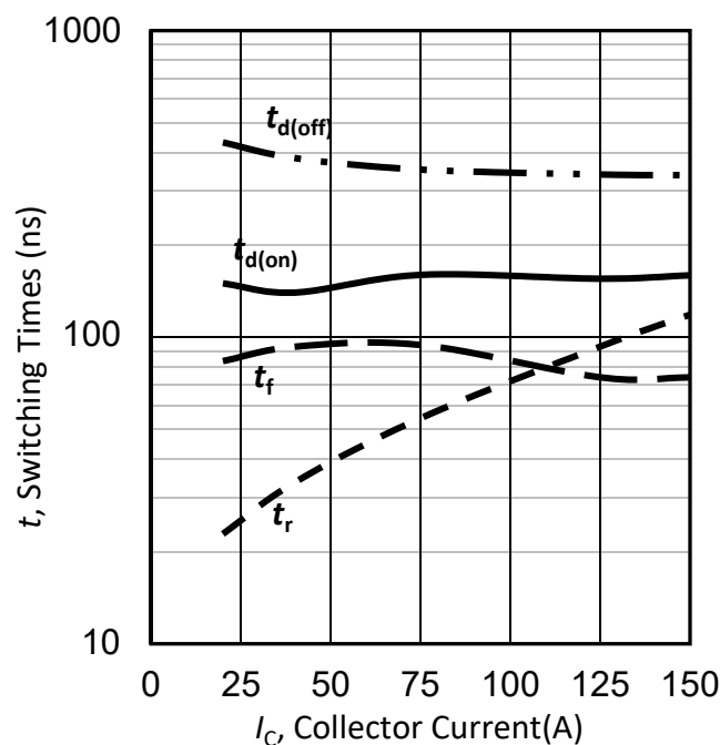
Figure 19. 典型开关时间与集电极电流的关系 /Typical switching times as a function of collector current (inductive load, T_{vj}=25^{\circ}\text{C} , V_{CE}=600\text{V} , V_{GE}=-5/17\text{V} , R_G=10\Omega )
