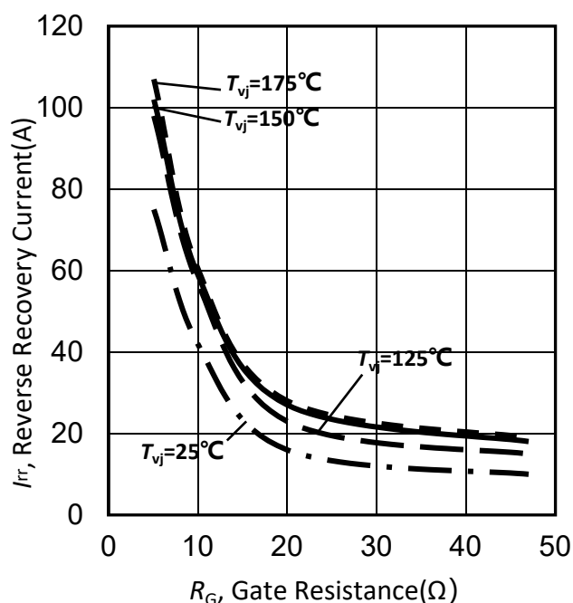
Figure 65. 典型反向恢复电流与栅极电阻器的关系 /Typical reverse recovery current as a function of gate resistor (inductive load, V_{CE}=600V , V_{GE}=-15/15V , I_C=75A )
