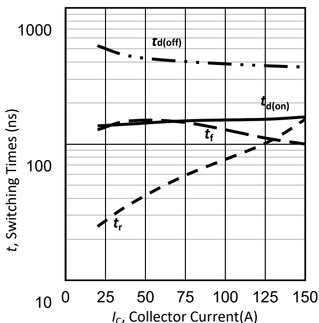
Figure 23. 典型开关时间与集电极电流的关系 /Typical switching times as a function of collector current (inductive load, T_{vj}=125^{\circ}\text{C} , V_{CE}=600\text{V} , V_{GE}=-5/17\text{V} , R_G=10\Omega )
