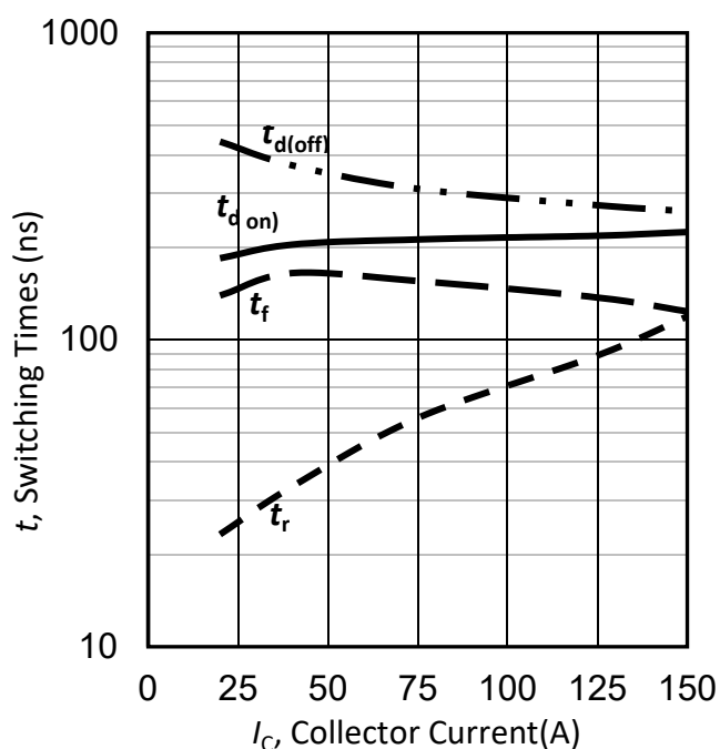
Figure 25. 典型开关时间与集电极电流的关系 /Typical switching times as a function of collector current (inductive load, T_{vj}=150^{\circ}\text{C} , V_{CE}=600\text{V} , V_{GE}=-15/15\text{V} , R_G=10\Omega )
