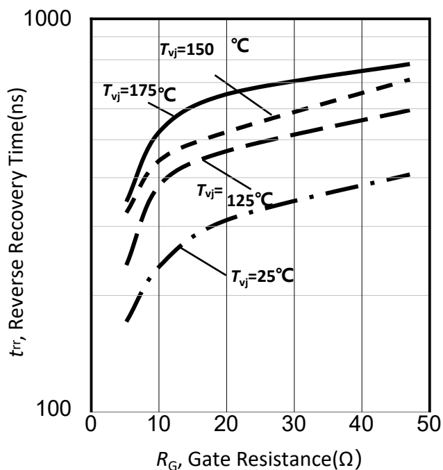
Figure 64. 典型反向恢复时间与栅极电阻器的关系/Typical reverse recovery time as a function of gate resistor (inductive load, V_{CE}=600V , V_{GE}=-5/17V , I_C=75A )
