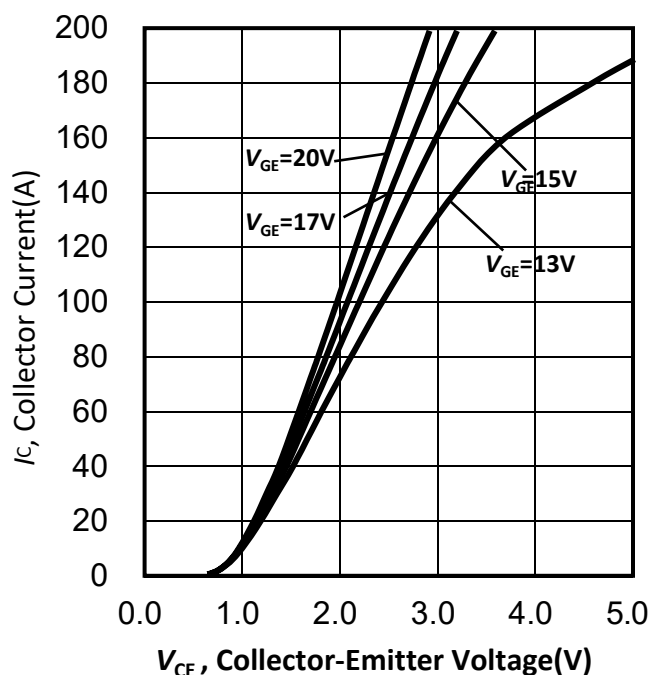
Figure 1. 典型输出特性/Typical output characteristic ( T_j=25^{\circ}\text{C} )
