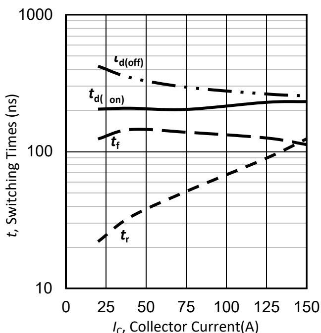
Figure 21. 典型开关时间与集电极电流的关系 /Typical switching times as a function of collector current (inductive load, T_{vj}=125^{\circ}\text{C} , V_{CE}=600\text{V} , V_{GE}=-15/15\text{V} , R_G=10\Omega )
