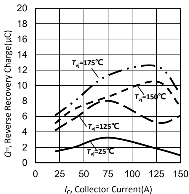
Figure 59. 典型反向恢复电荷与集电极电流的函数关系 /Typical reverse recovery charge as a function of collector current (inductive load, V_{CE}=600V, V_{GE}=-15/15V, R_G=10\Omega )
