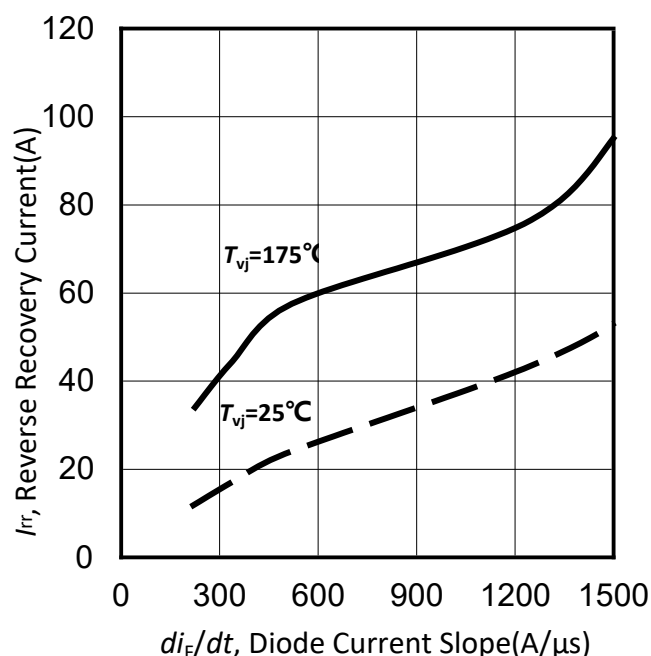
Figure 72. 典型反向恢复电流与二极管电流斜率的关系/Typical reverse recovery current as a function of diode current slope ( V_R=600V , I_F=75A )
