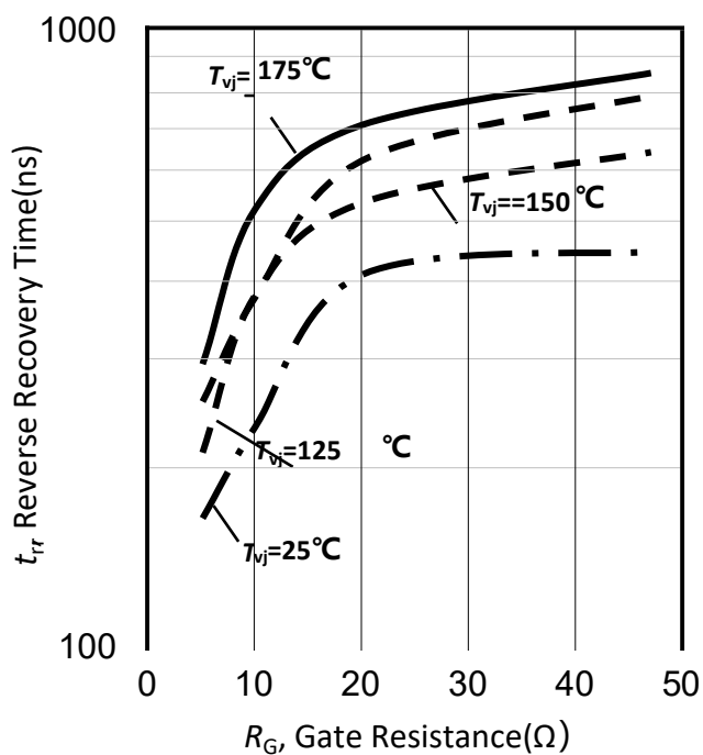
Figure 63. 典型反向恢复时间与栅极电阻器的关系/Typical reverse recovery time as a function of gate resistor (inductive load, V_{CE}=600V , V_{GE}=-15/15V , I_C=75A )
