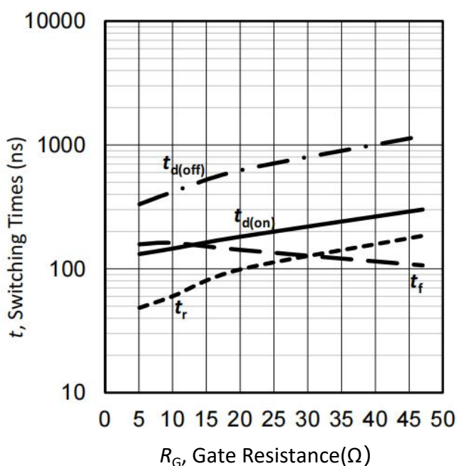
Figure 43. 典型开关时间与栅极电阻器的关系/Typical switching times as a function of gate resistor (inductive load, T_{vj}=150^{\circ}\text{C} , V_{CE}=600\text{V} , V_{GE}=-5/17\text{V} , I_C=75\text{A} )
