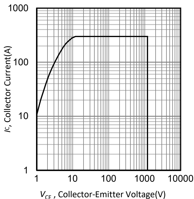
Figure 74. IGBT反向偏置安全工作区/IGBT reverse bias safe operating area ( T_{vj}\leq 175^\circ\text{C} , V_{GE}=15\text{V} )
