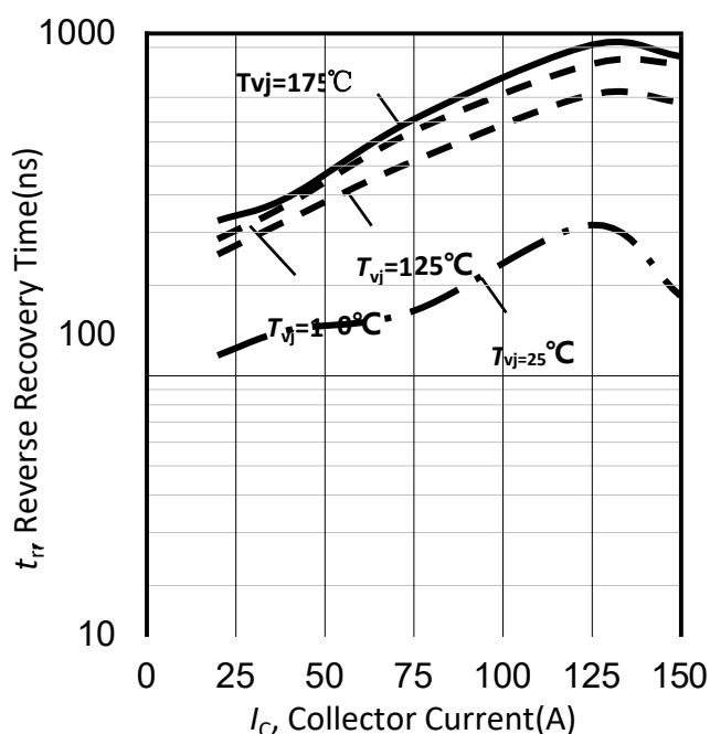
Figure 55. 典型反向恢复时间与集电极电流的关系/Typical reverse recovery time as a function of collector current (inductive load, V_{CE}=600V , V_{GE}=-15/15V , R_G=10\Omega )
