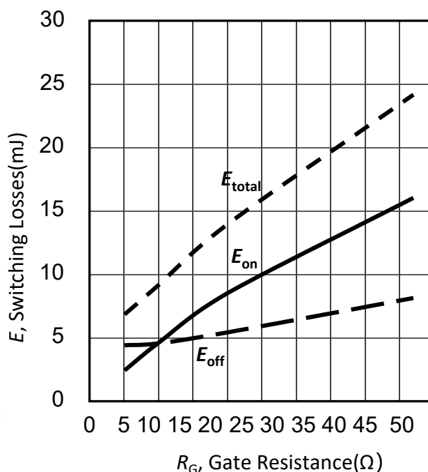
Figure 36. 典型开关时间与栅极电阻器的关系/Typical switching energy losses as a function of gate resistor(inductive load, T_{vj}=25^\circ\text{C} , V_{CE}=600\text{V} , V_{GE}=-5/17\text{V} , I_C=75\text{A} )
