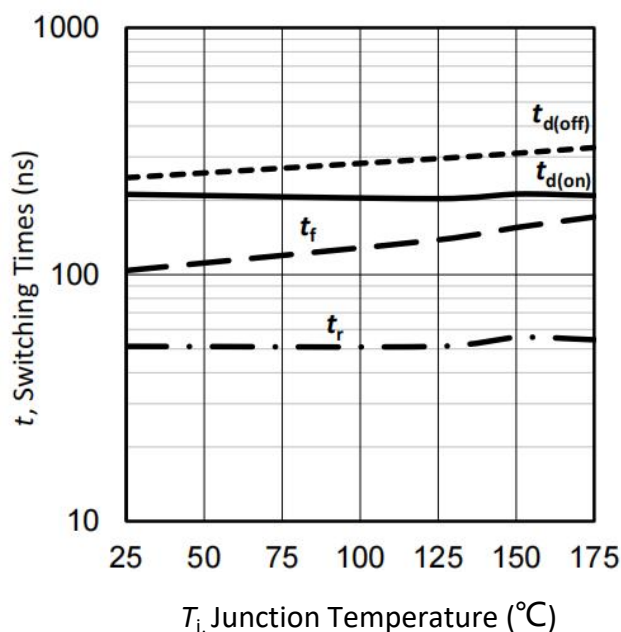
Figure 49. 典型开关时间与结温的关系/Typical switching times as a function of junction temperature (inductive load, V_{CE}=600V , V_{GE}=-15/15V , I_C=75A , R_G=10\Omega )
