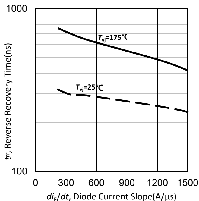
Figure 71. 典型反向恢复时间与二极管电流斜率的关系/Typical reverse recovery time as a function of diode current slope ( V_R=600V , I_F=75A )
