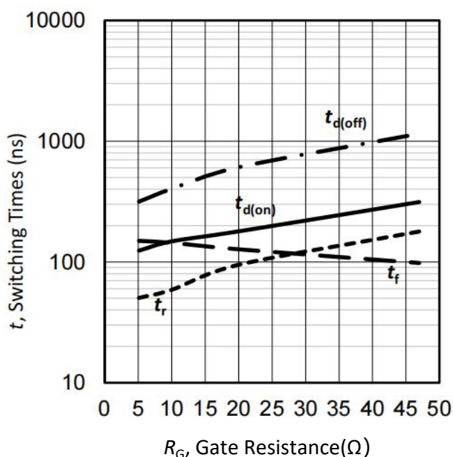
Figure 39. 典型开关时间与栅极电阻器的关系/Typical switching times as a function of gate resistor (inductive load, T_{vj}=125^{\circ}\text{C} , V_{CE}=600\text{V} , V_{GE}=-5/17\text{V} , I_C=75\text{A} )
