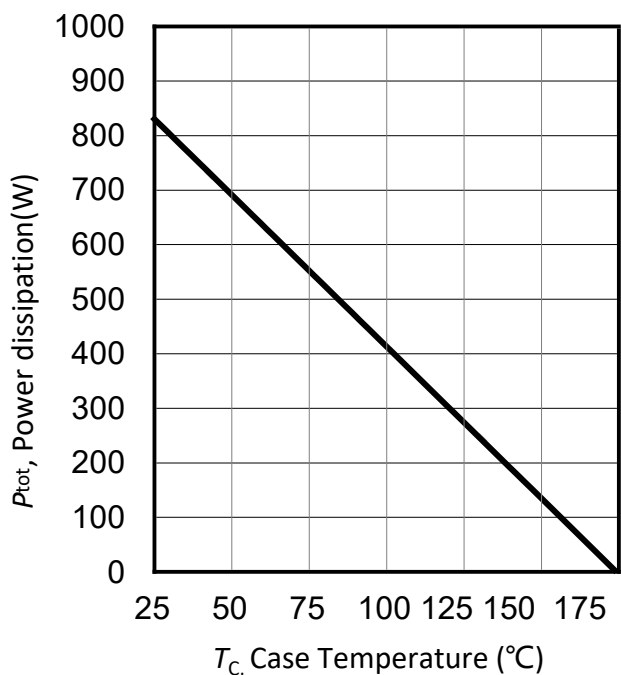
Figure 13. 功耗与外壳温度的关系/Power dissipation as a function of case temperature ( T_j \leq 175^\circ\text{C} )
