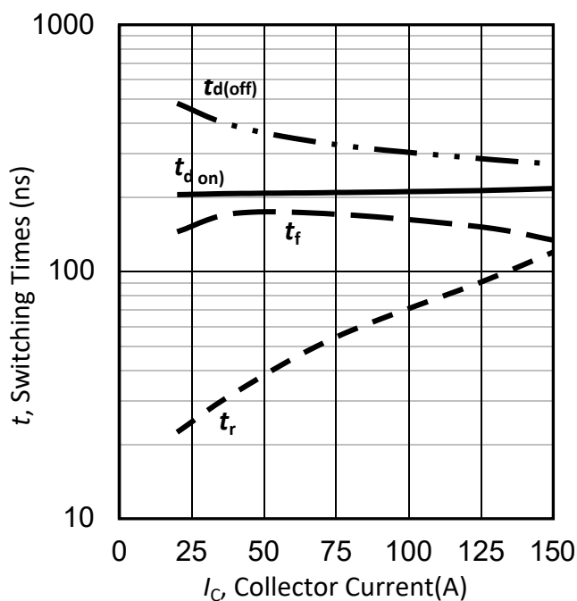
Figure 29. 典型开关时间与集电极电流的关系 /Typical switching times as a function of collector current (inductive load, T_{vj}=175^{\circ}\text{C} , V_{CE}=600\text{V} , V_{GE}=-15/15\text{V} , R_G=10\Omega )
