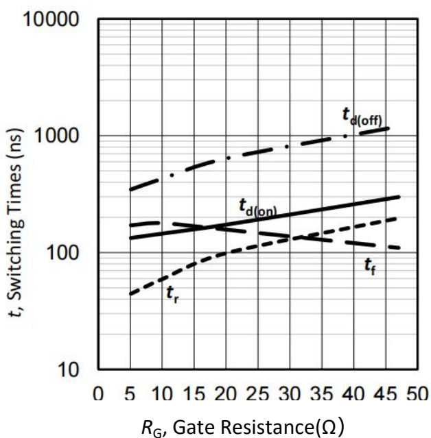
Figure 47. 典型开关时间与栅极电阻器的关系/Typical switching times as a function of gate resistor (inductive load, T_{vj}=175^{\circ}\text{C} , V_{CE}=600\text{V} , V_{GE}=-5/17\text{V} , I_C=75\text{A} )
