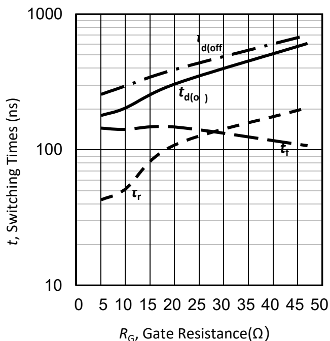
Figure 37. 典型开关时间与栅极电阻器的关系/Typical switching times as a function of gate resistor (inductive load, T_{vj}=125^{\circ}\text{C} , V_{CE}=600\text{V} , V_{GE}=-15/15\text{V} , I_C=75\text{A} )
