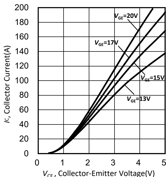
Figure 4. 典型输出特性/Typical output characteristic ( T_j=175^{\circ}\text{C} )
