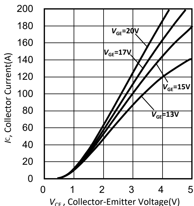
Figure 3. 典型输出特性/Typical output characteristic ( T_j=150^{\circ}\text{C} )
