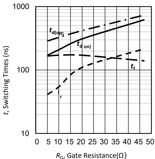
Figure 45. 典型开关时间与栅极电阻器的关系/Typical switching times as a function of gate resistor (inductive load, T_{vj}=175^{\circ}\text{C} , V_{CE}=600\text{V} , V_{GE}=-15/15\text{V} , I_C=75\text{A} )
