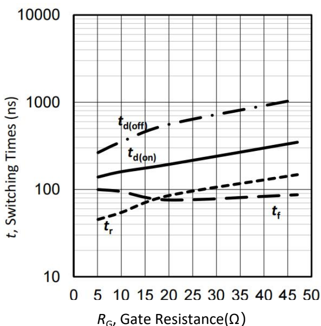
Figure 35. 典型开关时间与栅极电阻器的关系/Typical switching times as a function of gate resistor (inductive load, T_{vj}=25^\circ\text{C} , V_{CE}=600\text{V} , V_{GE}=-5/17\text{V} , I_C=75\text{A} )
