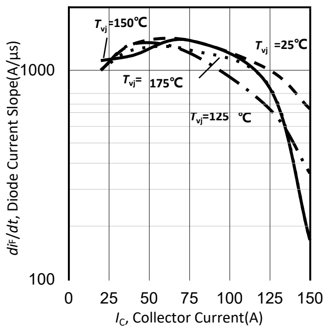
Figure 61. 典型二极管电流斜率与集电极电流的函数关系/Typical diode current slope as a function of collector current (inductive load, V_{CE}=600V , V_{GE}=-15/15V , R_G=10\Omega )
