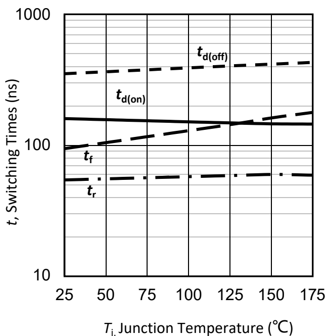
Figure 51. 典型开关时间与结温的关系/ Typical switching times as a function of junction temperature (inductive load, V_{CE}=600V , V_{GE}=-5/17V , I_C=75A , R_G=10\Omega )
