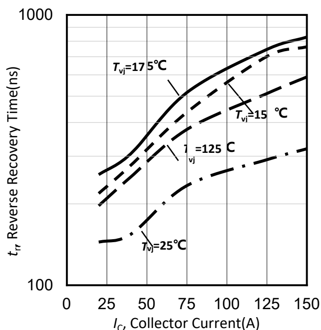
Figure 56. 典型反向恢复时间与集电极电流的关系 //Typical reverse recovery time as a function of collector current (inductive load, V_{CE}=600V , V_{GE}=-5/17V , R_G=10\Omega )
