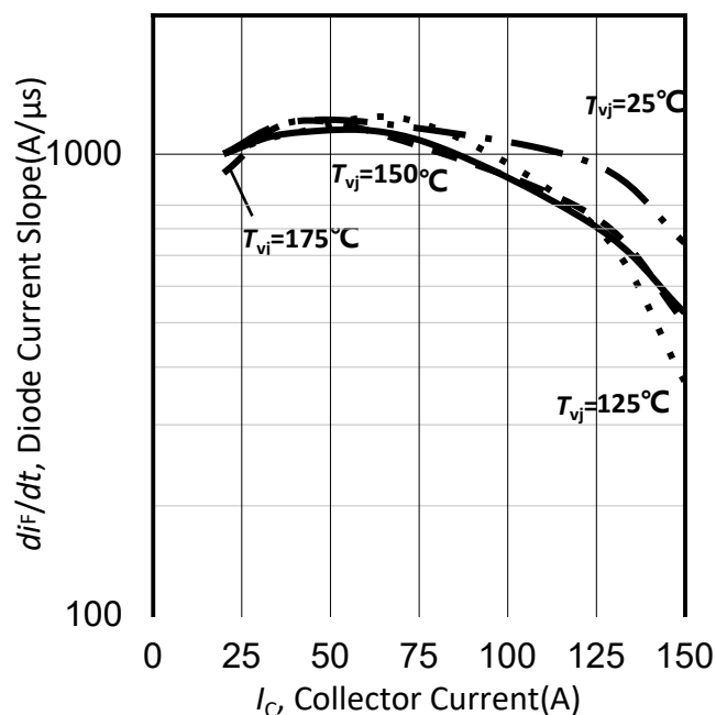
Figure 62. 典型二极管电流斜率与集电极电流的函数关系/Typical diode current slope as a function of collector current (inductive load, V_{CE}=600V , V_{GE}=-5/17V , R_G=10\Omega )
