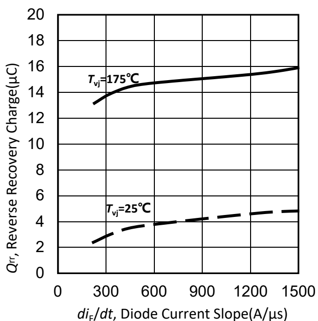
Figure 73. 典型反向恢复电荷与二极管电流斜率的关系/Typical reverse recovery charge as a function of diode current slope ( V_R=600\text{V} , I_F=75\text{A} )
