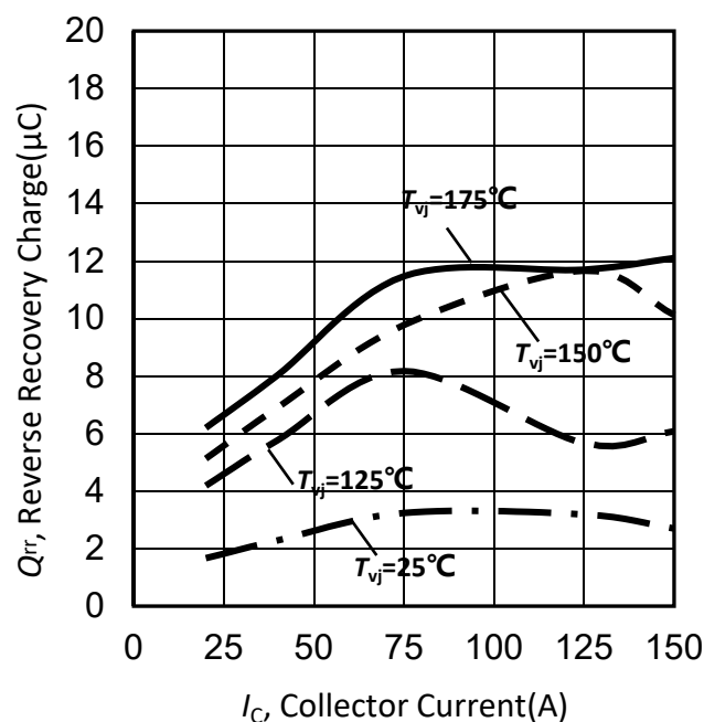
Figure 60. 典型反向恢复电荷与集电极电流的函数关系 /Typical reverse recovery charge as a function of collector current (inductive load, V_{CE}=600V, V_{GE}=-5/17V, R_G=10\Omega )
