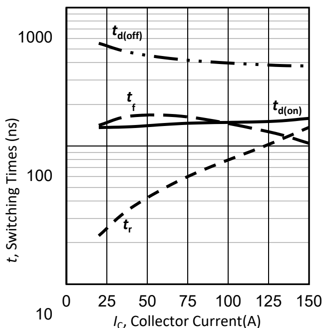
Figure 27. 典型开关时间与集电极电流的关系 /Typical switching times as a function of collector current (inductive load, T_{vj}=150^{\circ}\text{C} , V_{CE}=600\text{V} , V_{GE}=-5/17\text{V} , R_G=10\Omega )
