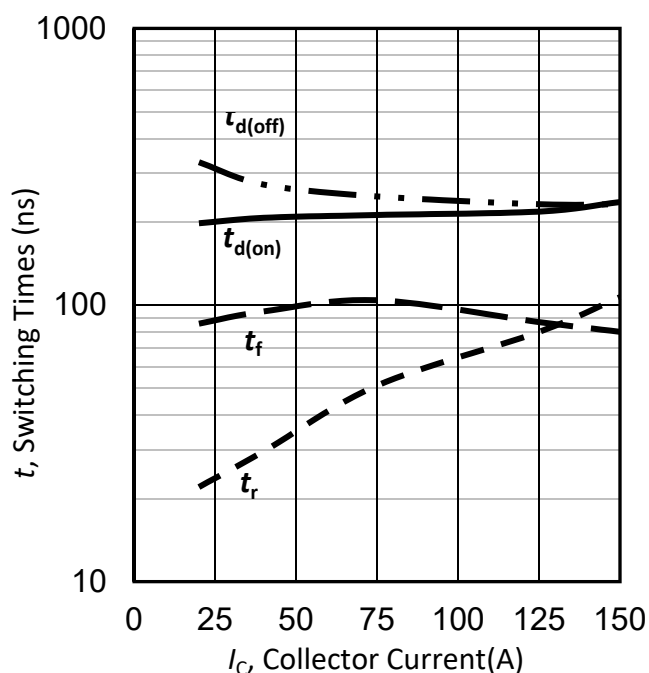
Figure 17. 典型开关时间与集电极电流的关系 /Typical switching times as a function of collector current (inductive load, T_{vj}=25^{\circ}\text{C} , V_{CE}=600\text{V} , V_{GE}=-15/15\text{V} , R_G=10\Omega )
