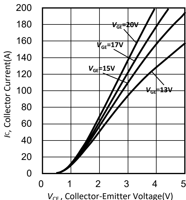
Figure 2. 典型输出特性/Typical output characteristic ( T_j=125^{\circ}\text{C} )
